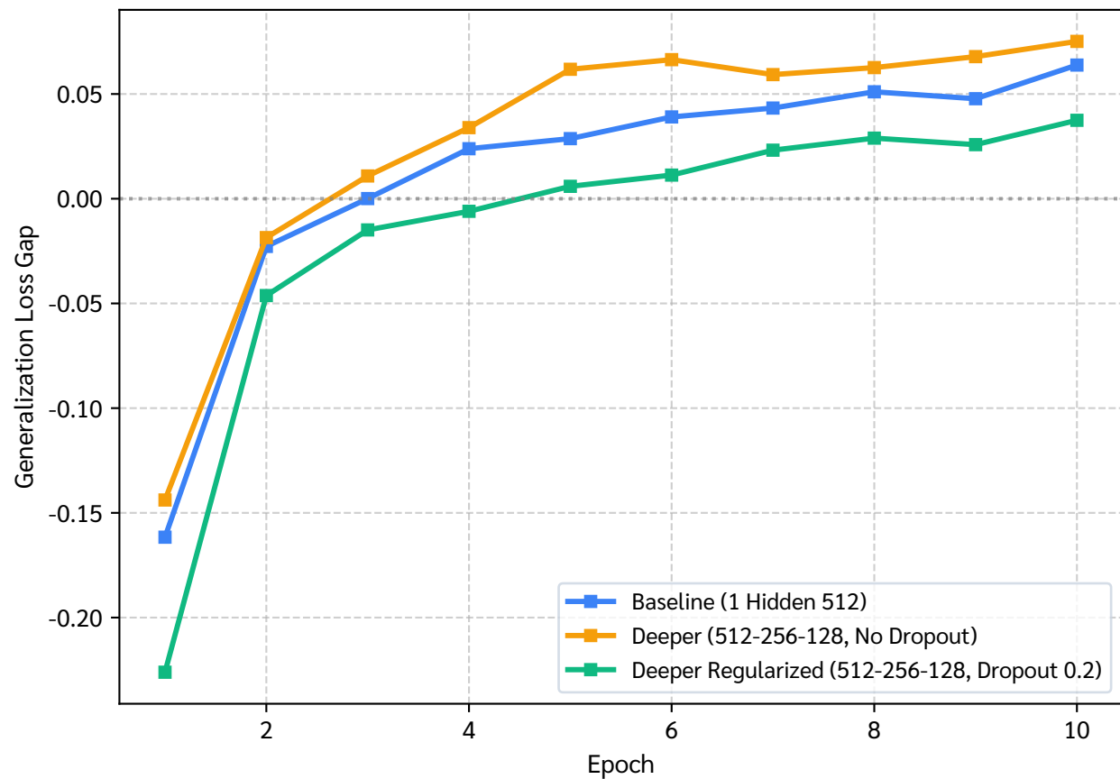
Generalization Gap (Validation Loss - Training Loss)
