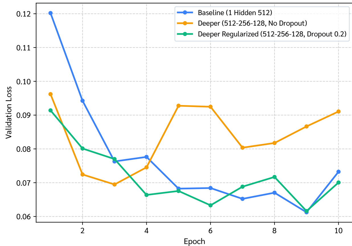
Validation Loss: Baseline vs. Deeper Architectures
